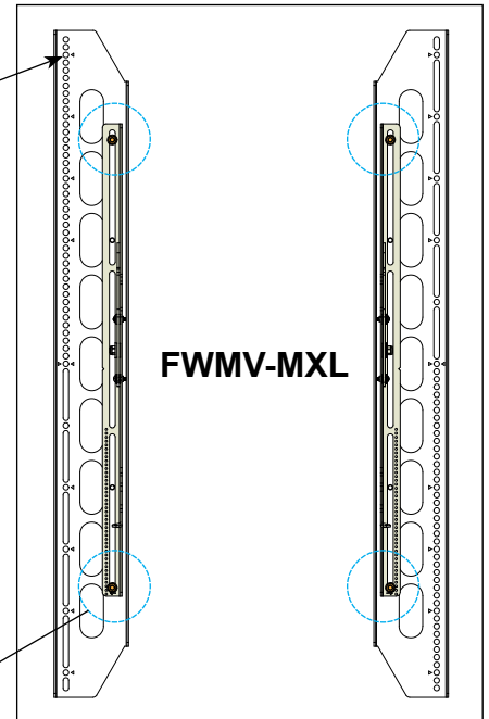
M8 Flat Washer (4 pcs)
